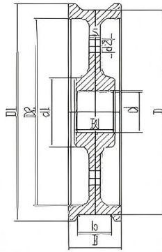
Double Flange
